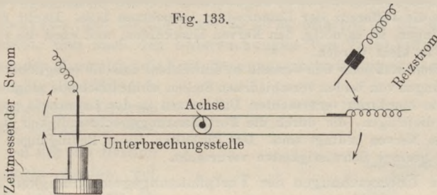
Helmholtz'sche Wippe.
