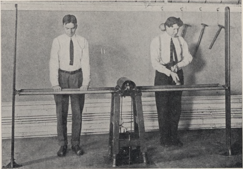
Fig. 224.—The vibrating bars (Kellogg).
