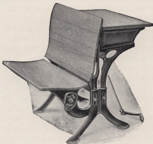
Figs. 130 and 131.—The Peabody sanitary adjustable desk. One bolt on each side is loosened and the crank inserted and turned, thus raising or lowering the desk or seat as required. (Courtesy of Garden City Educational Co., Chicago, Illinois.)
