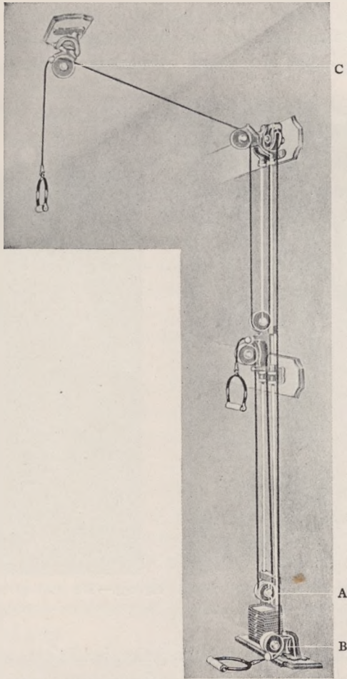
Fig. 231.—Triplex pulley-weight (Narragansett Co.).
