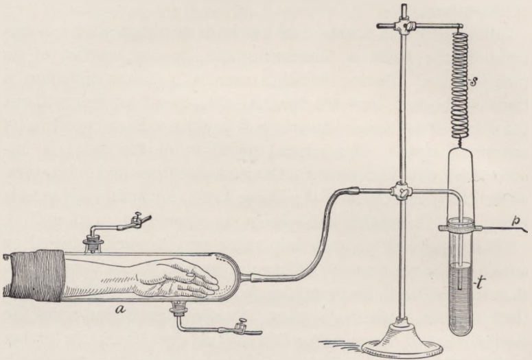
Fig. 10.—A schematic diagram of Mosso's plethysmograph for the arms: a , The glass cylinder for the arm, with rubber sleeve and two tubulatures for filling with warm water; s , the spiral spring swinging the test-tube t . The spring is so calibrated that the level of the liquid in the test-tube above the arm remains unchanged as the tube is filled and emptied. The movements of the tube are recorded on a drum by the writing point p (Howell).
