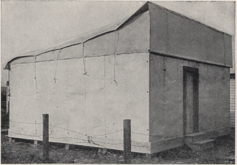
Fig. 112.—Portable bath-house used in Baltimore, Md. The outside (courtesy of Playground Association of America).
