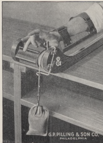
Fig. 241.—The finger treadmill.
